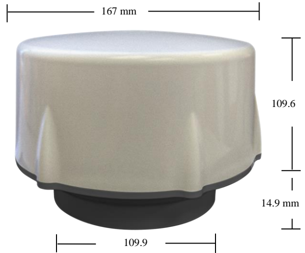
VeraPhase 6000 Dimensions (mm) Conical Radome also available
